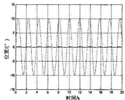
图6 稳定平台隔离扰动图 Fig.6 Disturbances isolation of stabilized platform
