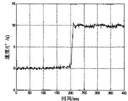
图5 \omega_0 = 10 (°)/s 时速度环响应 Fig.5 Rate response at \omega_0 = 10 (°)/s
