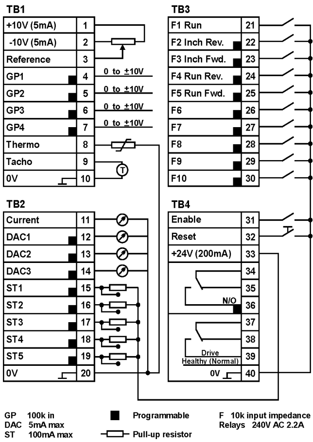
15 Control connections.
